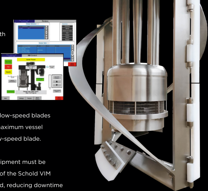
Top Left: VIM HMI Screens Top Right: VIM with Helical Arms and Scrapers
